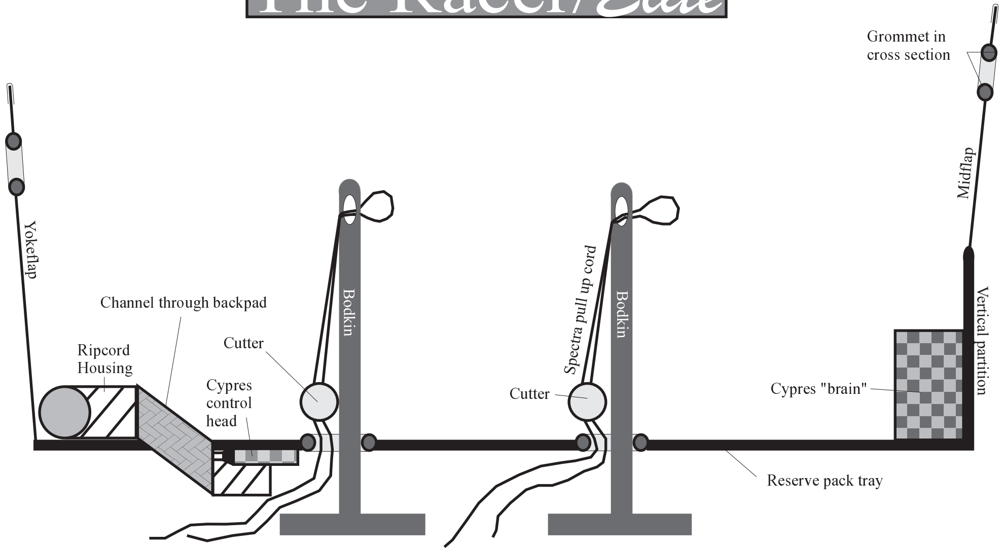
Figure 2: Racer/Elite series pack tray in cross section (center slice)
